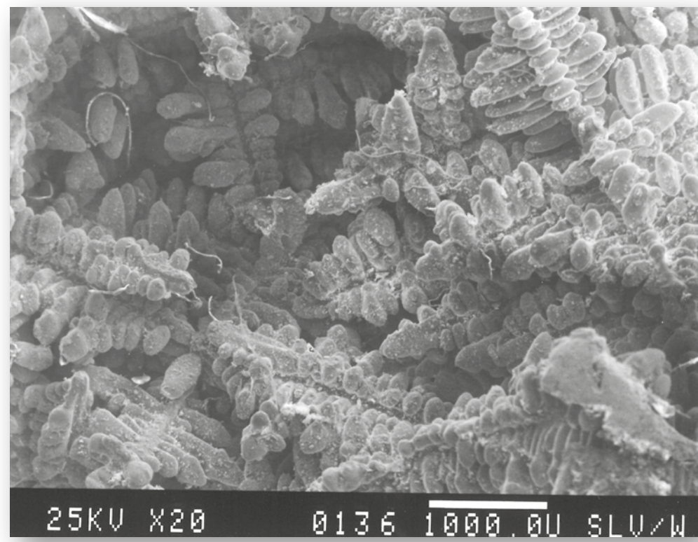
Lunker
