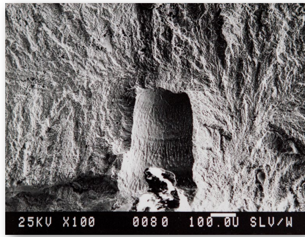
metallurgische Pore
