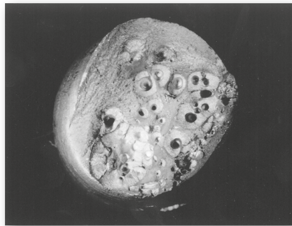
metallurgische Pore
